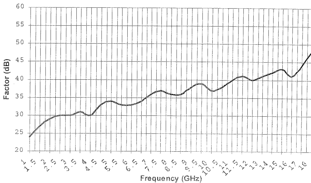
Figure 1-1 Typical Antenna Factors
