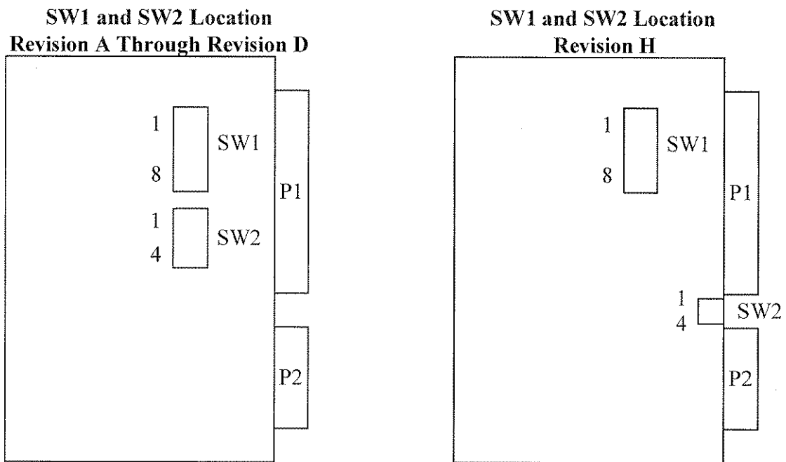
Figure 2-1 Address Switches
