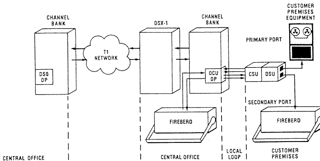
Figure 1-7 Straightaway Test Configuration
