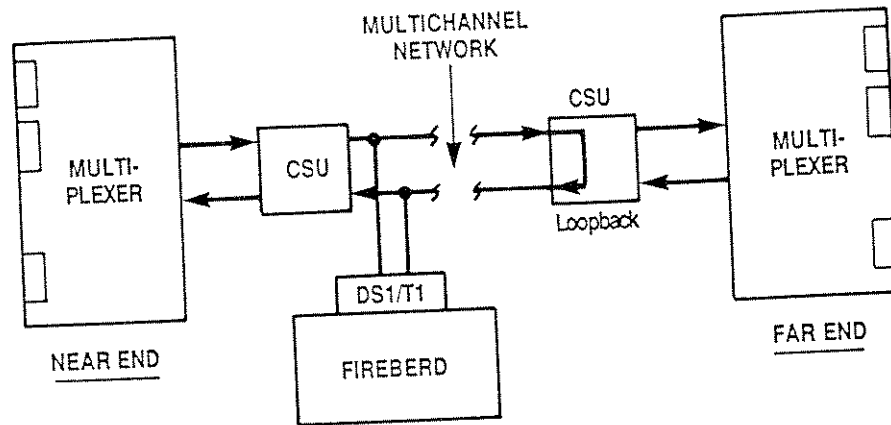
Figure 1-15 Remote Loopback Test
