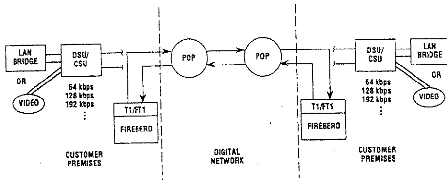
Figure 1-12 End-To-End Fractional T1 Testing
